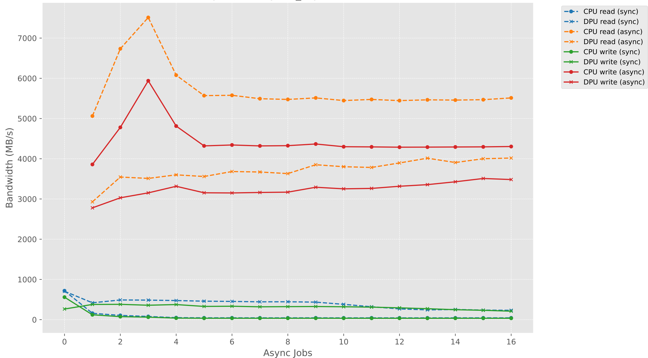
Bandwidth vs Async Jobs (sync1_asyncN) - SEQ (CPU vs DPU)
